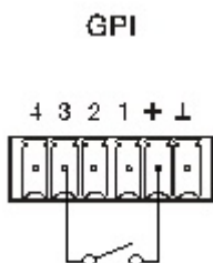
Example of connection: GPI 3
